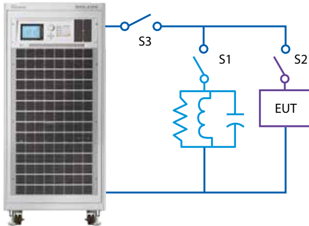
61800 Series Regenerative Grid Simulator
